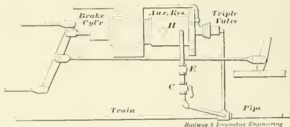
RECHARGING DEVICE ATTACHED TO FREIGHT BRAKE.
